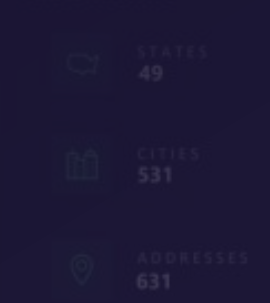
REGION STATS
